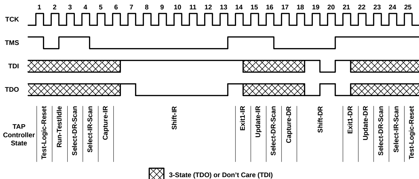
Figure 4. Timing Example
